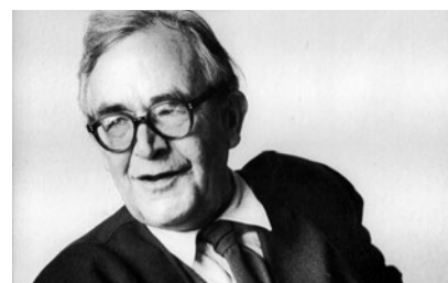
Karl Barth, 1886–1968
